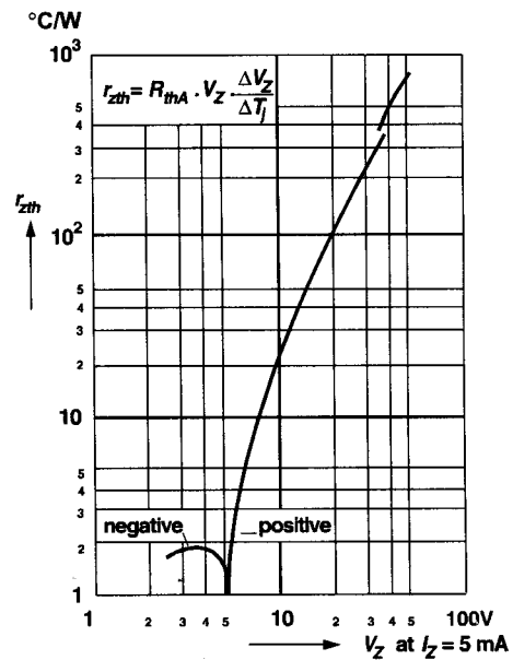
Thermal differential resistance versus Zener voltage
