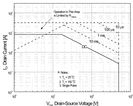
Figure 9-1. Maximum Safe Operating Area for IRF840B
