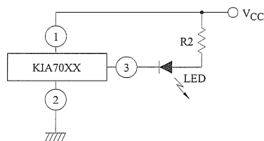
(1) BATTERY LOW INDICATOR
