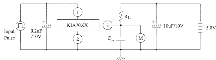
APPLICATION CIRCUIT
