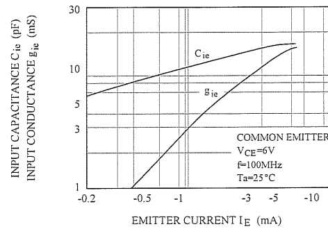
C_{ie}, g_{ie} - I_E
