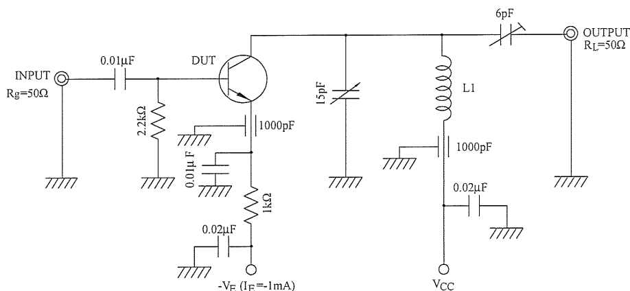
Fig. G_{pe} TEST CIRCUIT
