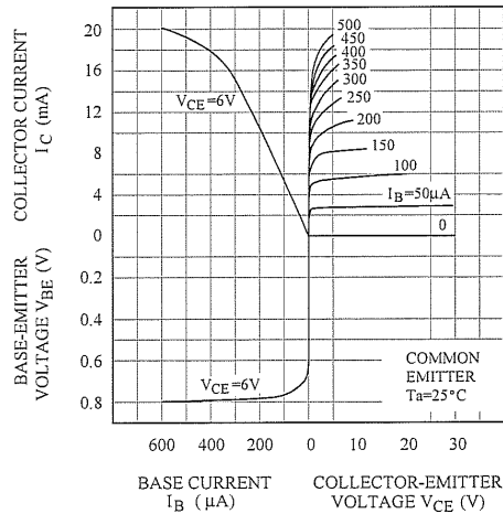
STATIC CHARACTERISTICS
