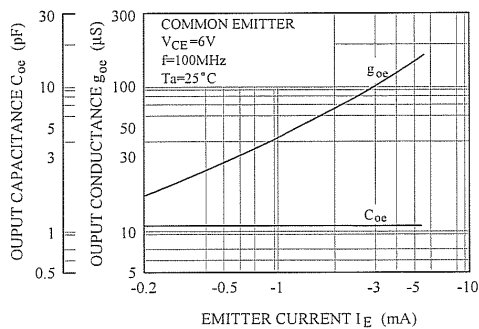
C_{oe}, g_{oe} - I_E
