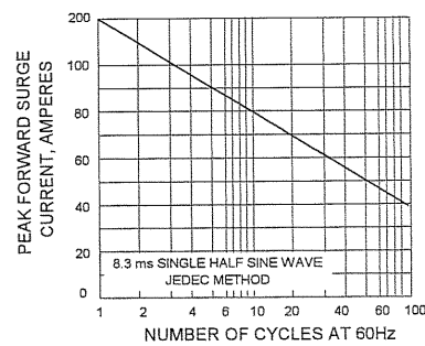
FIG.2 - MAXIMUM NON-REPETITIVE SURGE CURRENT
