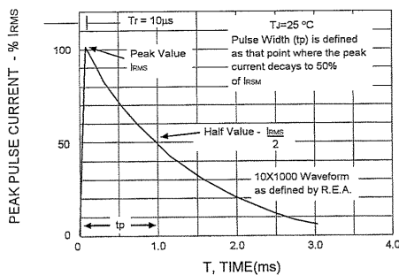
FIG.5 - PULSE WAVEFORM
