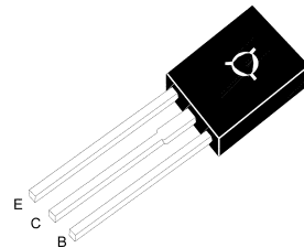
TO-18 Plastic Package
