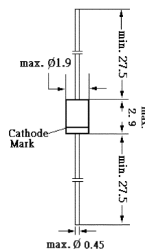
Glass case JEDEC DO-34 Dimensions in mm
