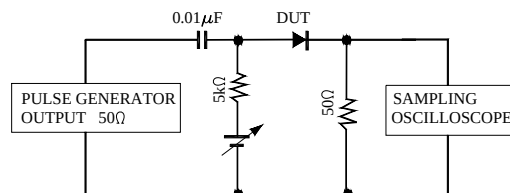
Reverse Recovery Time Measurement Circuit
