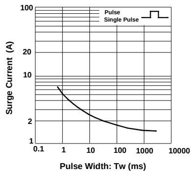
Surge Current Characteristics
