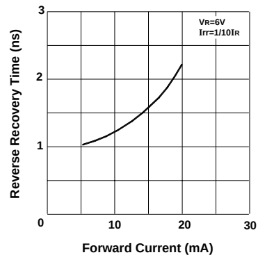
Reverse Recovery Time Characteristics
