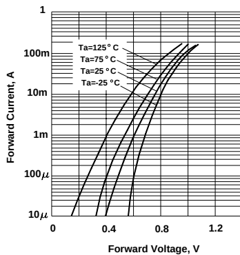
Forward Characteristics
