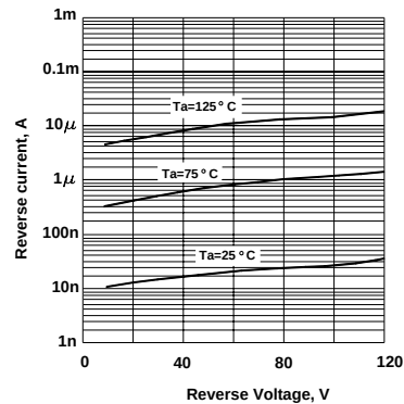
Reverse Characteristics
