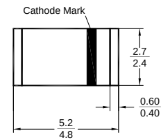
Plastic case MELF (DO-213AB) Dimensions in mm
