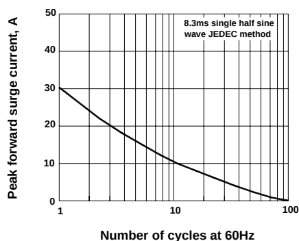
Maximum non-repetitive forward surge current
