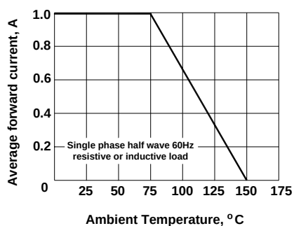
Typical forward current derating curve
