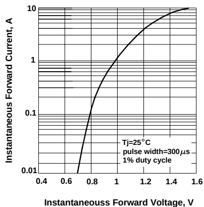
Typical Instantaneous Forward Characteristics
