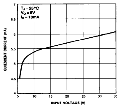
Figure 4. Quiescent Current
