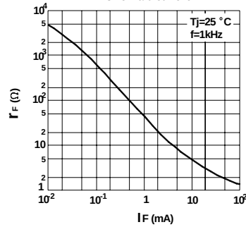
Dynamic forward resistance vs. forward current
