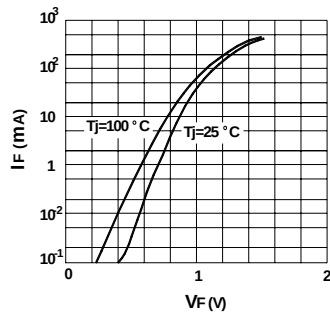
Forward characteristics
